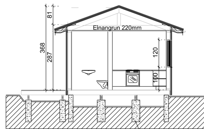
SNID B-B
